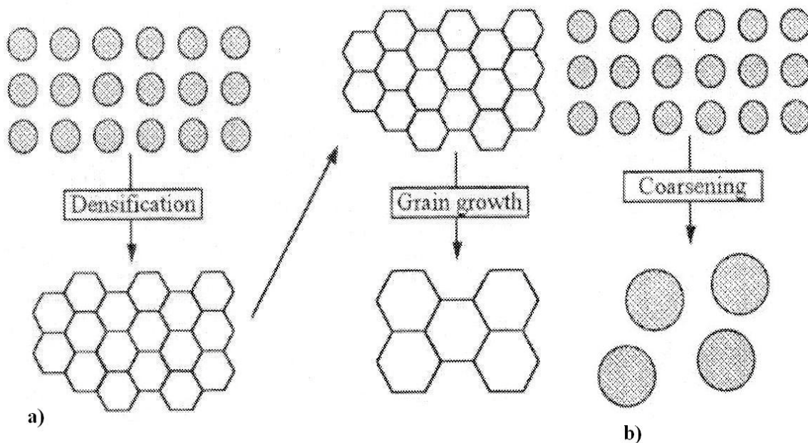
Figure 4.3 Frittage en phase solide, a) Densification, b) Coalescence.
